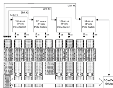
▲ 2 3 4 5 6 7 8 9 • Backplane Link Configuration
