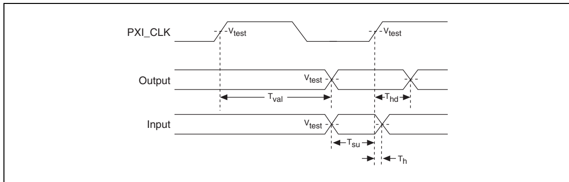
Figure 4-2. PXI Synchronous Trigger Timing
